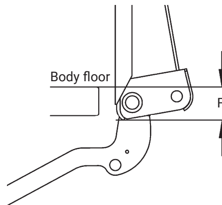
Abbildung 29. The platforms overlap (F)
