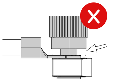
Figure 84. Montage erroné
