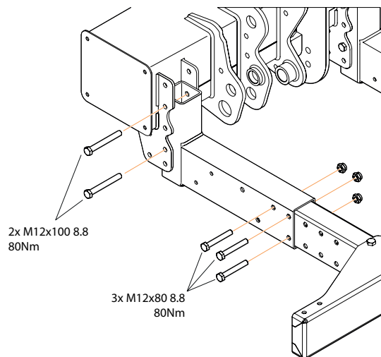
Figure 51. Pose de la protection anti-encastrement
